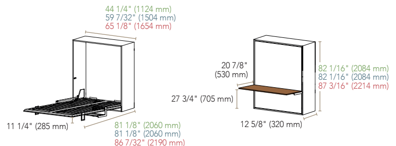
The dimensions shown in the drawings are the overall dimensions with 3/4" (19 mm) panel.
