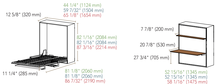
The dimensions shown in the drawings are the overall dimensions with 3/4" (19 mm) panel.
