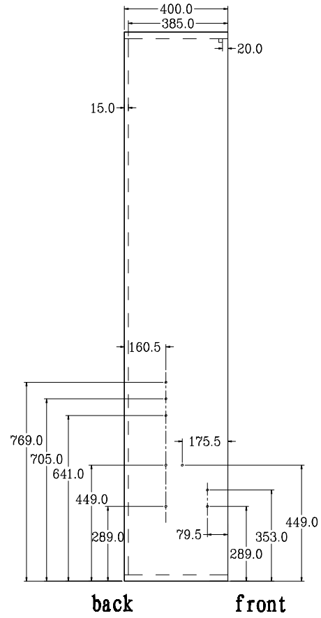
Hole drilling guideline for bracket mounting
