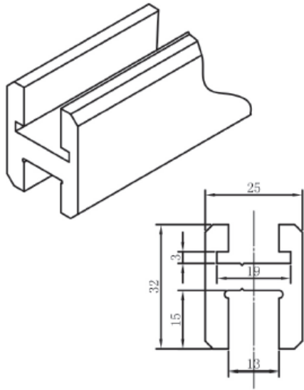
Header extrusion
