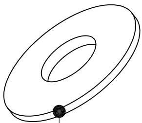
gasket \phi 30 * \phi 11.2 * 1.5
