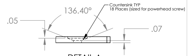
DETAIL A SCALE 1 : 1.5
