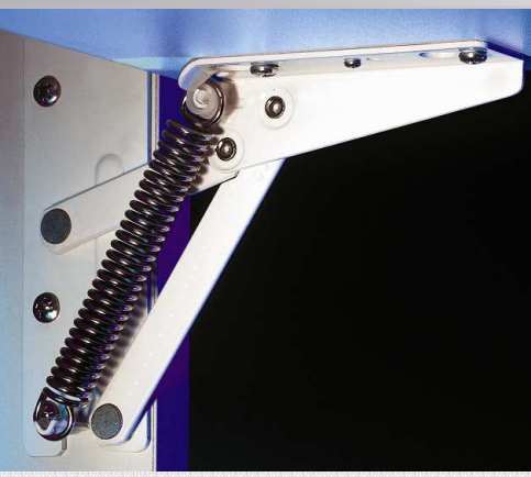
542L30 – Left flap fitting
