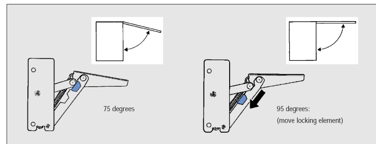
One fitting - two opening angles
