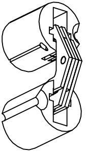
HINGE OPEN 180° CHARNIÈRE OUVERTE 180° ISOMETRIC VIEW
