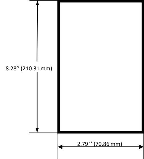
SSSM3ENDCAP5XXX
