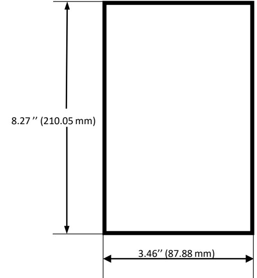
SSSM5ENDCAP1XX
