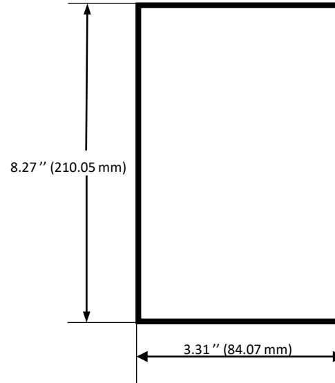
SSSM4ENDCAP1XX
