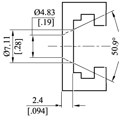
HOLE DETAIL
