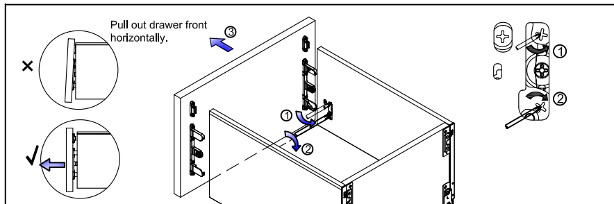
Release drawer front
