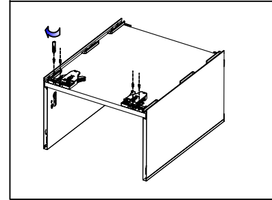
Locking Brackets assembly
