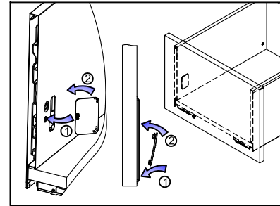
Cover Cap assembly
