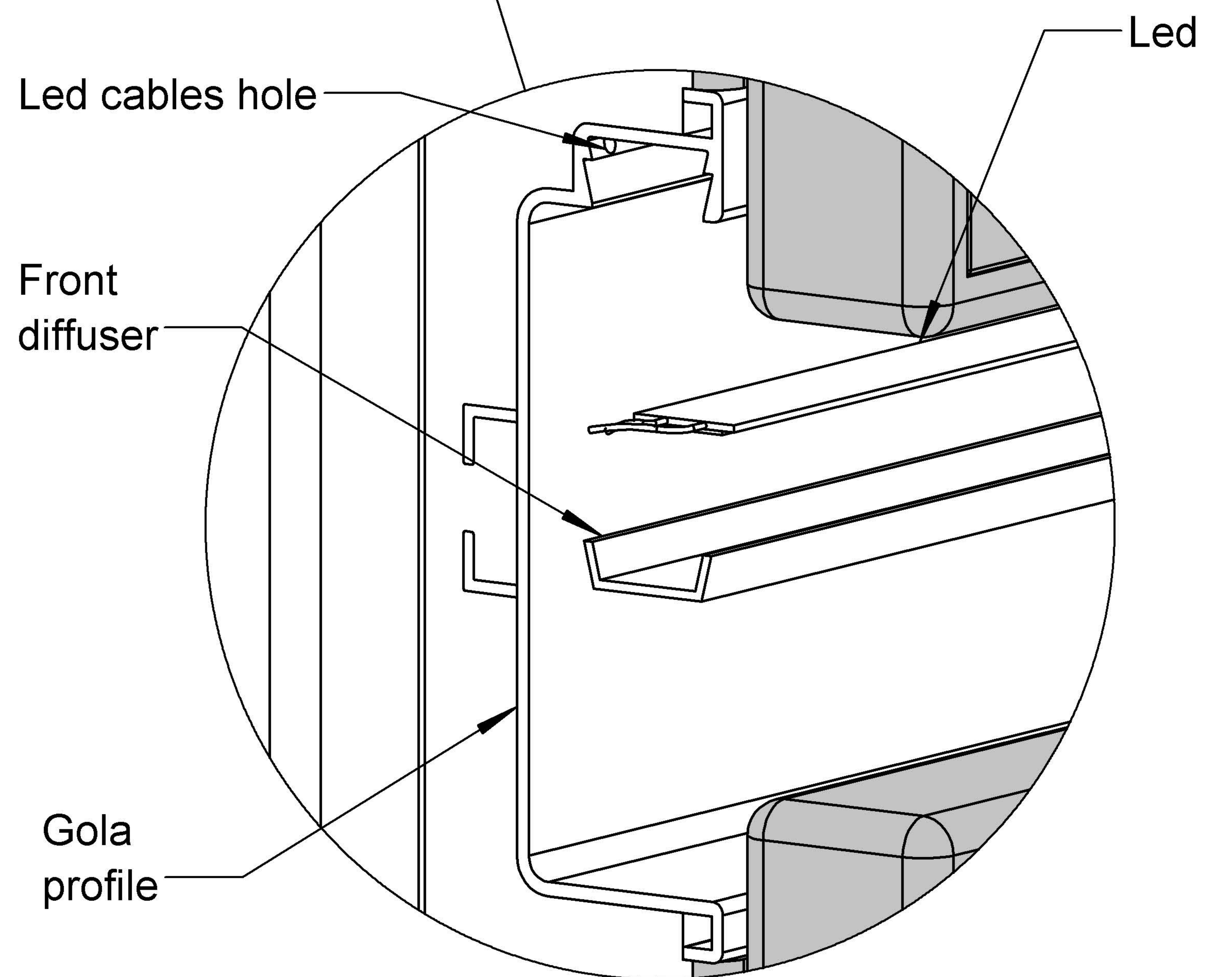
LED DISASSEMBLY
