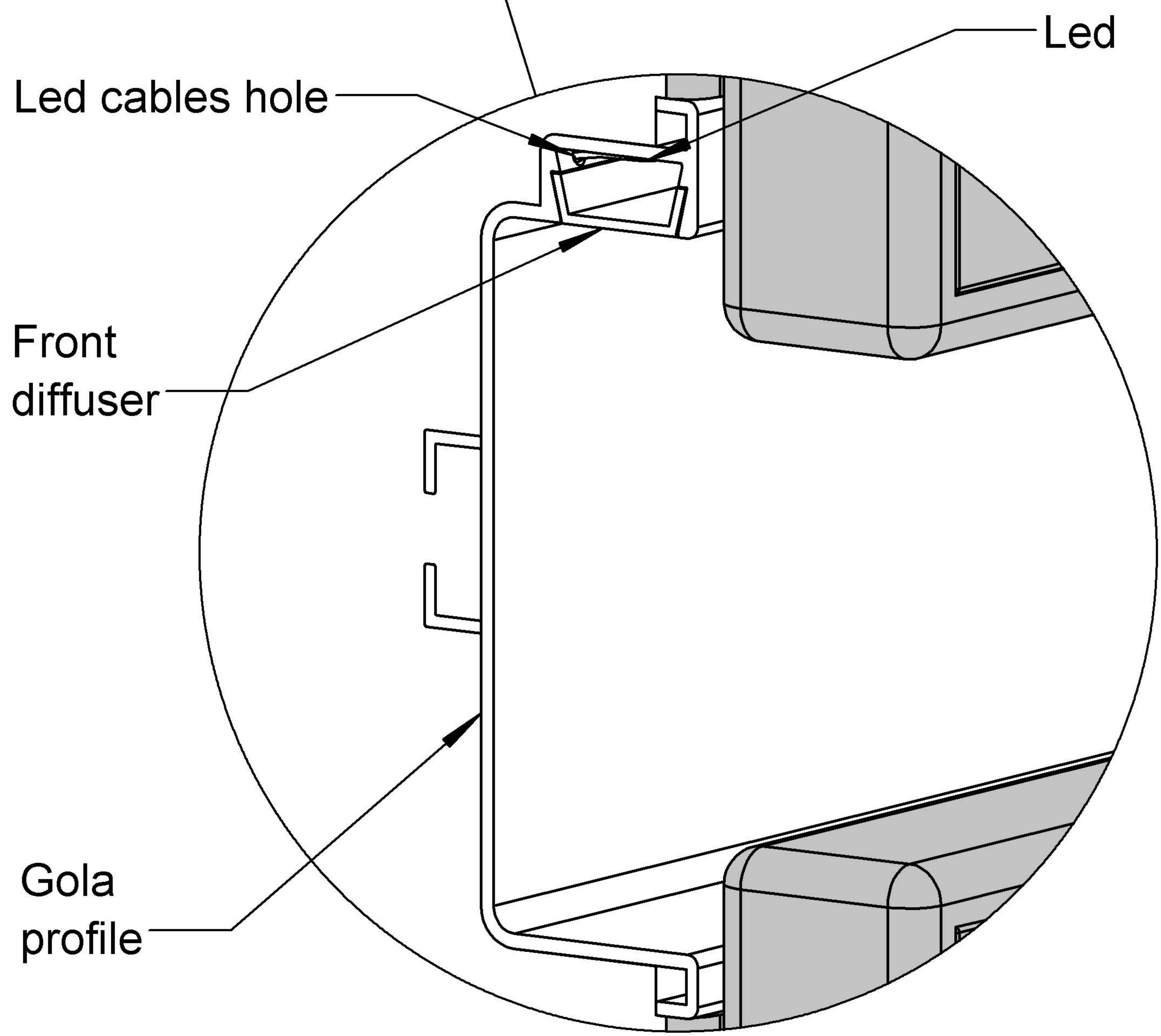
LED ASSEMBLY
