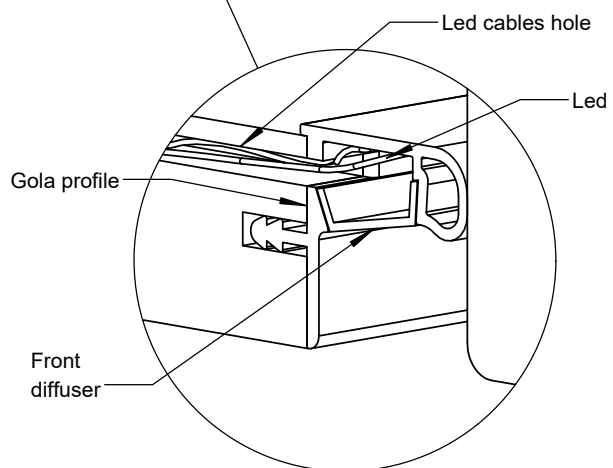
LED ASSEMBLY
