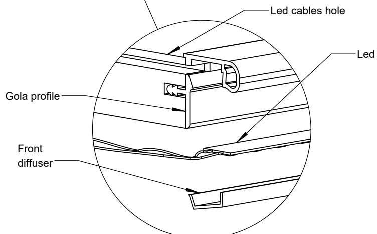
LED DISASSEMBLY
