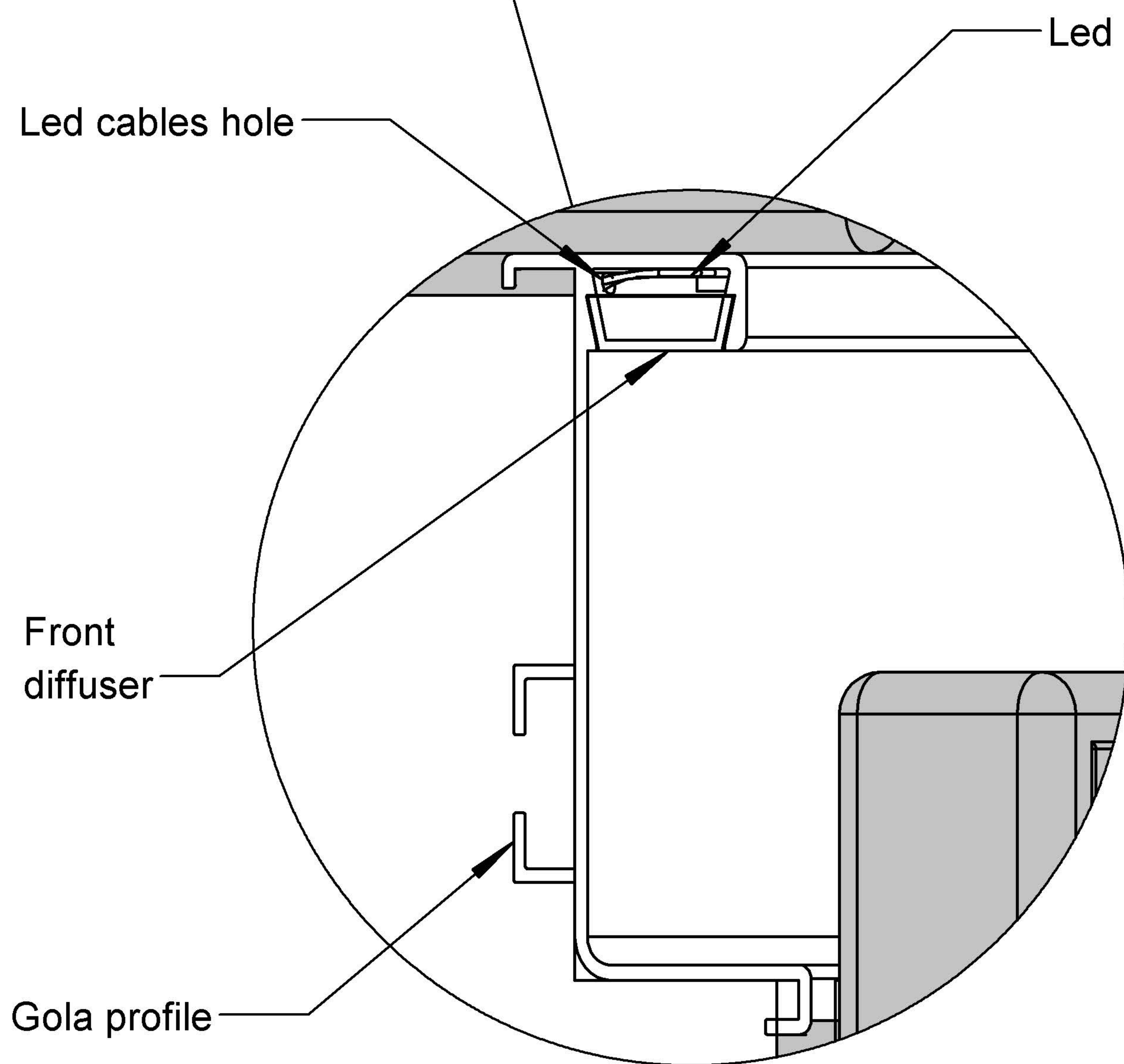
LED ASSEMBLY
