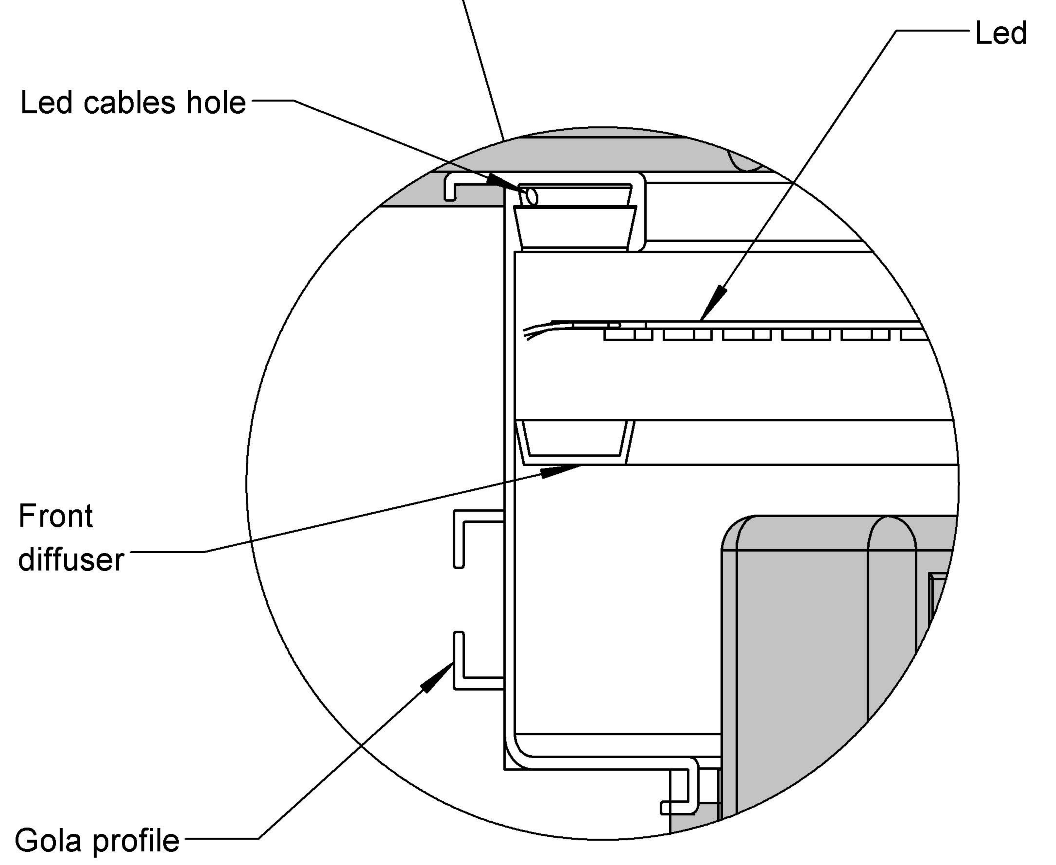
LED DISASSEMBLY
