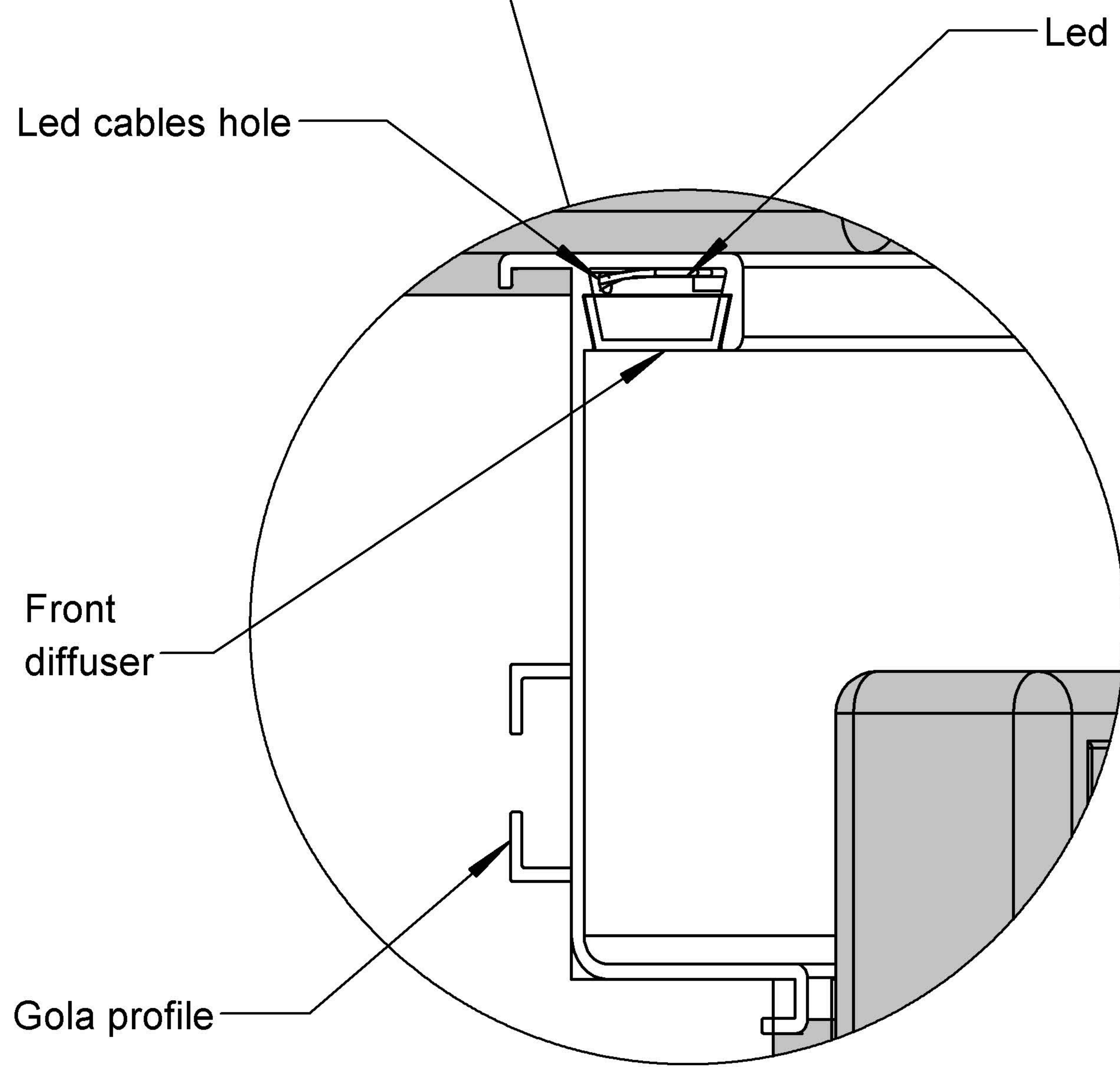
LED ASSEMBLY
