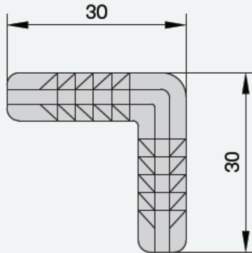
Angular dowel 90° 8 mm dia hole
