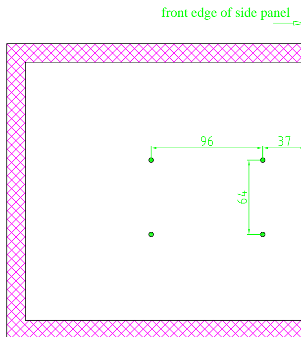
Installing hole position
