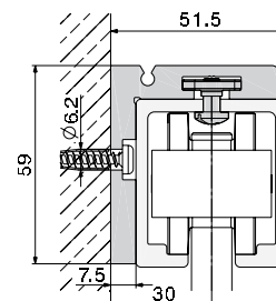
HAWA-Junior 120 cristal
