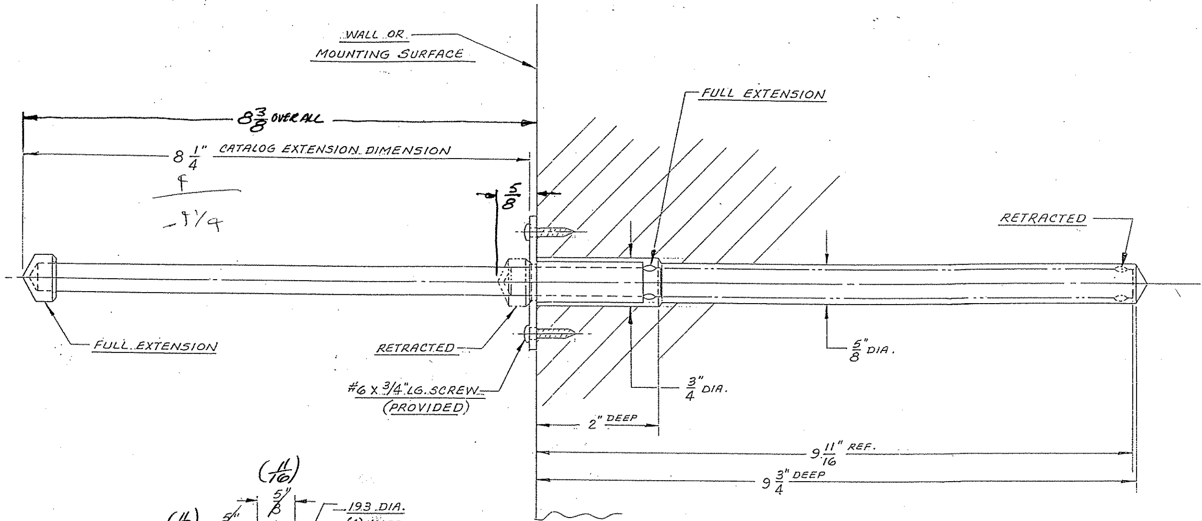
CROSS SECTION THROUGH MOUNTING WALL SHOWING CLEARANCES REQUIRED
