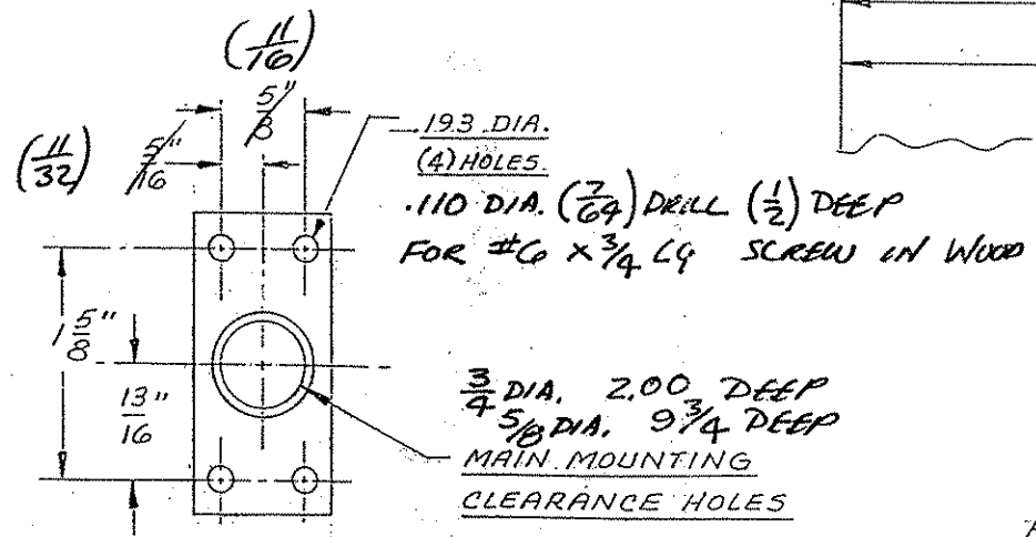
HOLE PATTERN OF PLATE
