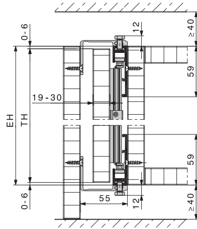
Système : HAWA-Concepta 25/30 Raccordement : Connector 55 mm System: HAWA-Concepta 25/30 Connection: Connector 55 mm
