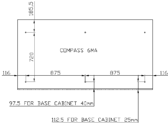
HOLES CABINET DOOR
