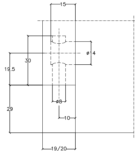
Detail E; scale 1 : 1
